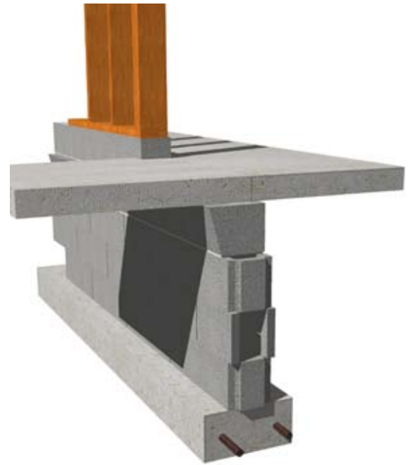
Section at Garage
